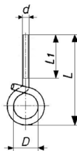
Rope loop open
